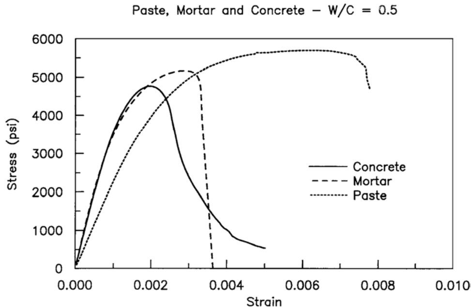
Fig. 2.2—Stress-strain curves for cement paste, mortar, and concrete; w/c = 0.5 (Martin, Darwin, and Terry 1991).
