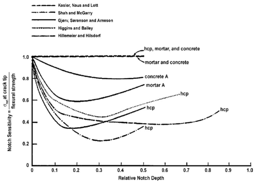
Fig. 2.6—Effect of relative notch depth on notch sensitivity (based on data from Higgins and Bailey 1976; Kesler, Naus, and Lott 1972; Shah and McGarry 1971; Gjörv, Sorenson, and Arneson 1977; Hillemeier and Hilsdorf 1977).
