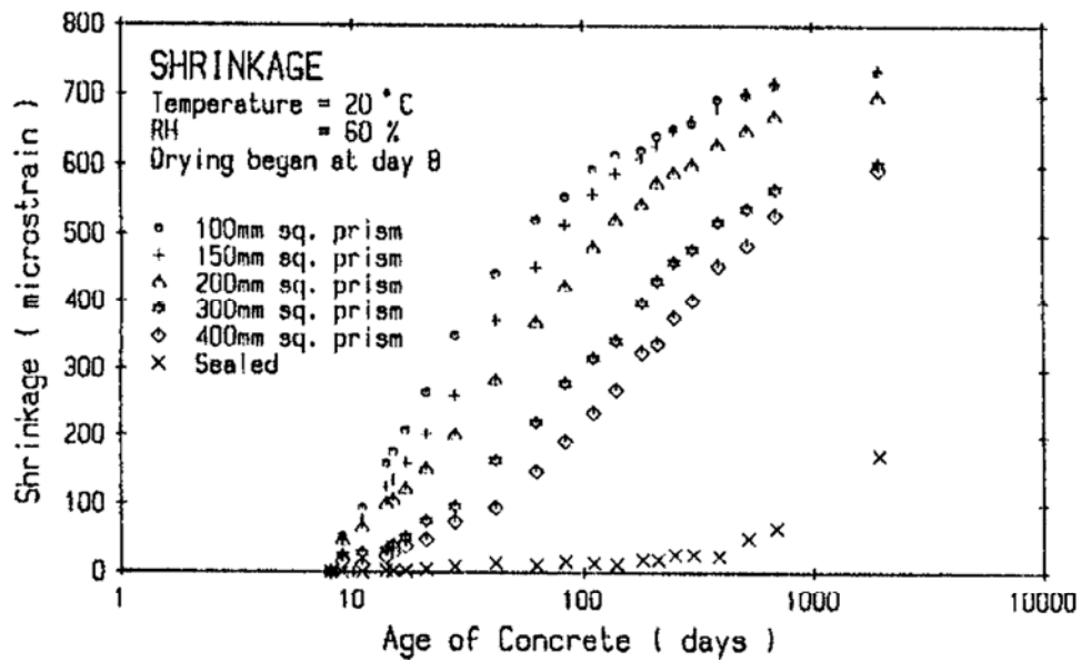
Fig. 3.8—Influence of specimen size on shrinkage (Bryant and Vadhanavikkitt 1987).
